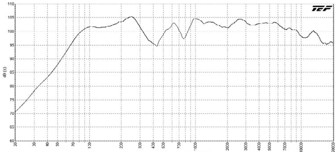
AH6565S Frequency Response
